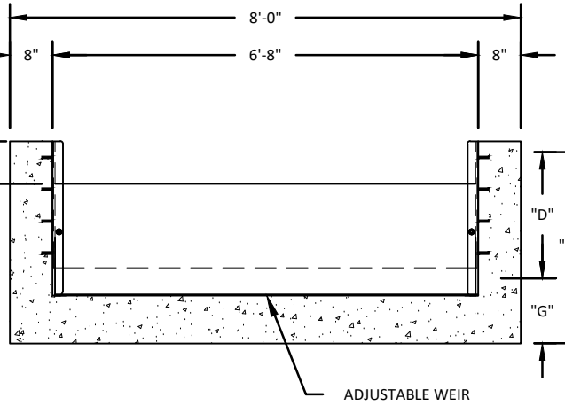
ADJUSTABLE WEIR - TYPICAL
