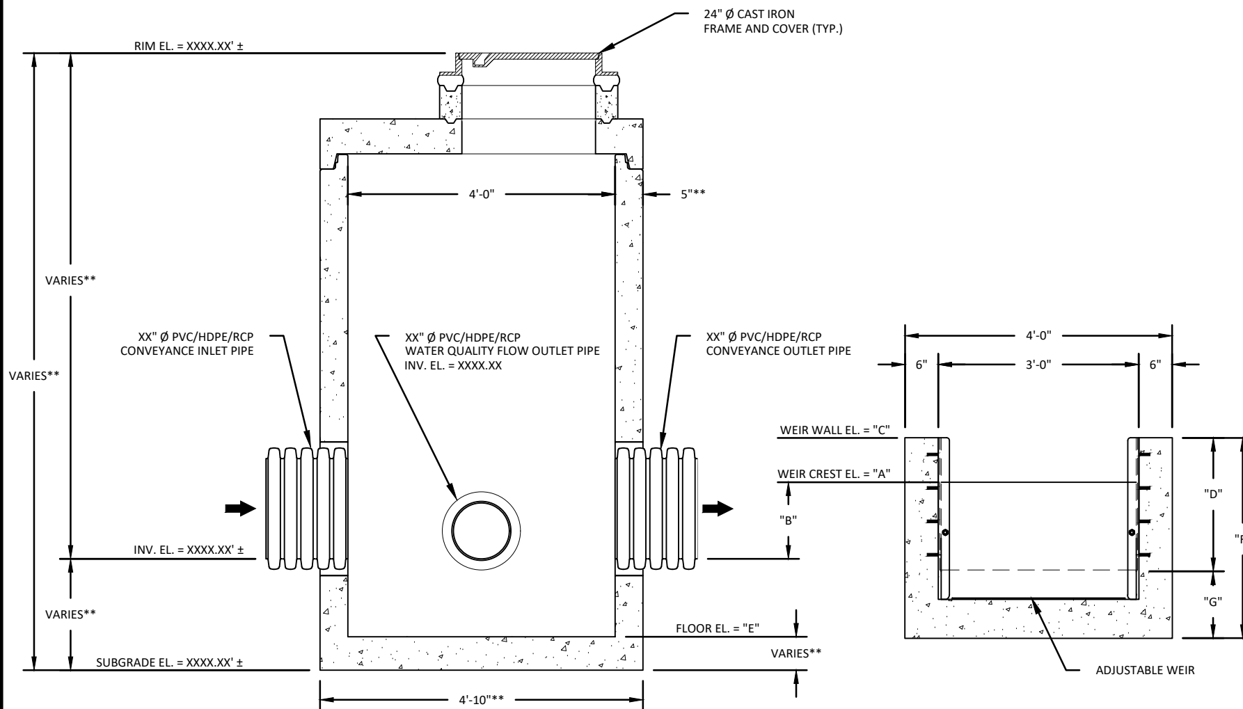
SECTION A-A - ADJUSTABLE WEIR NOT SHOWN FOR CLARITY
