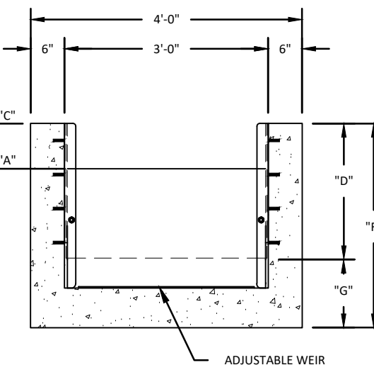
ADJUSTABLE WEIR - TYPICAL
