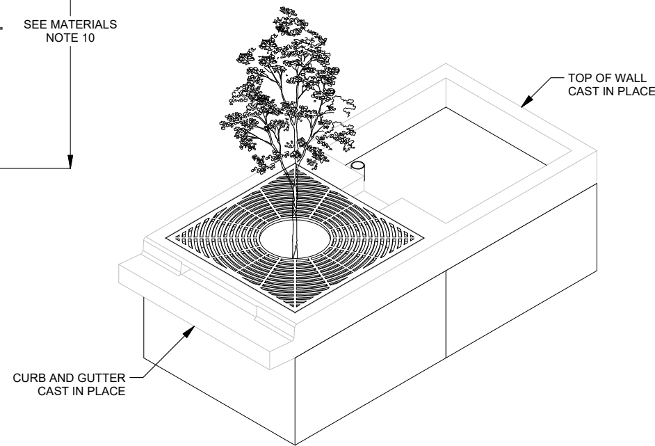
ISOMETRIC VIEW
