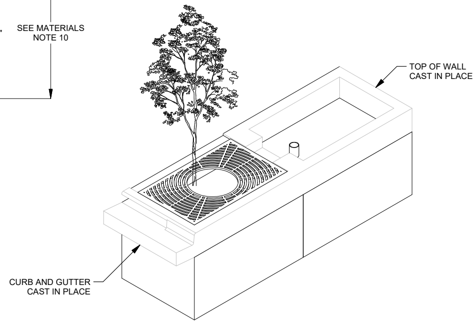
ISOMETRIC VIEW
