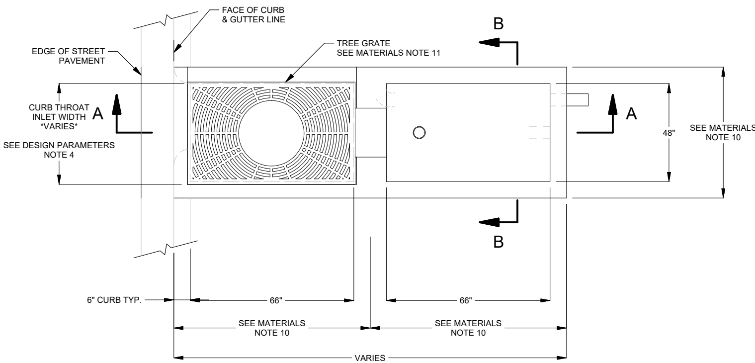
PLAN VIEW
