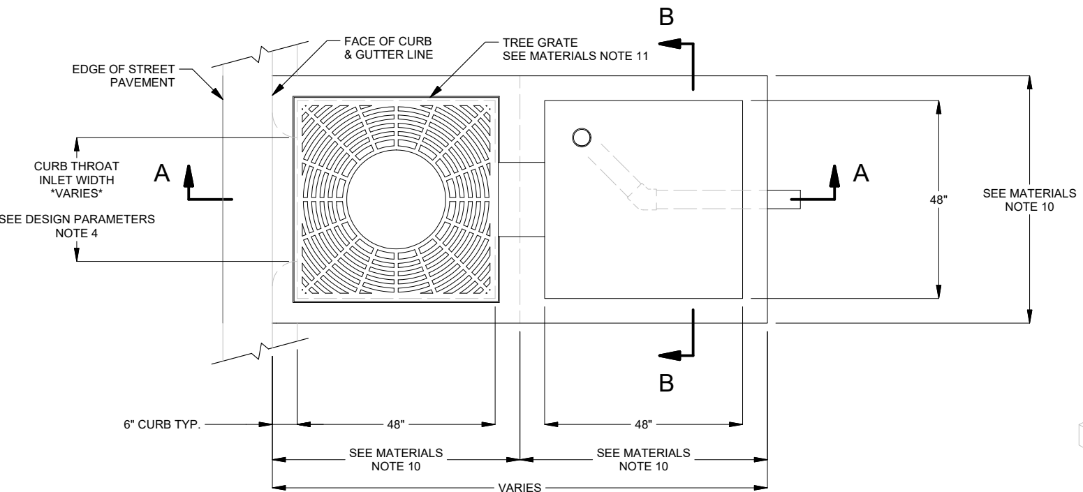
PLAN VIEW
