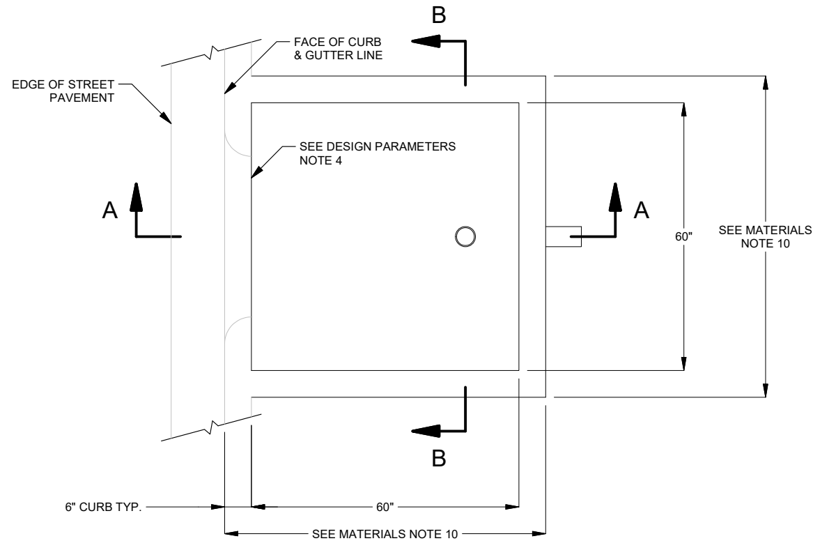
PLAN VIEW
