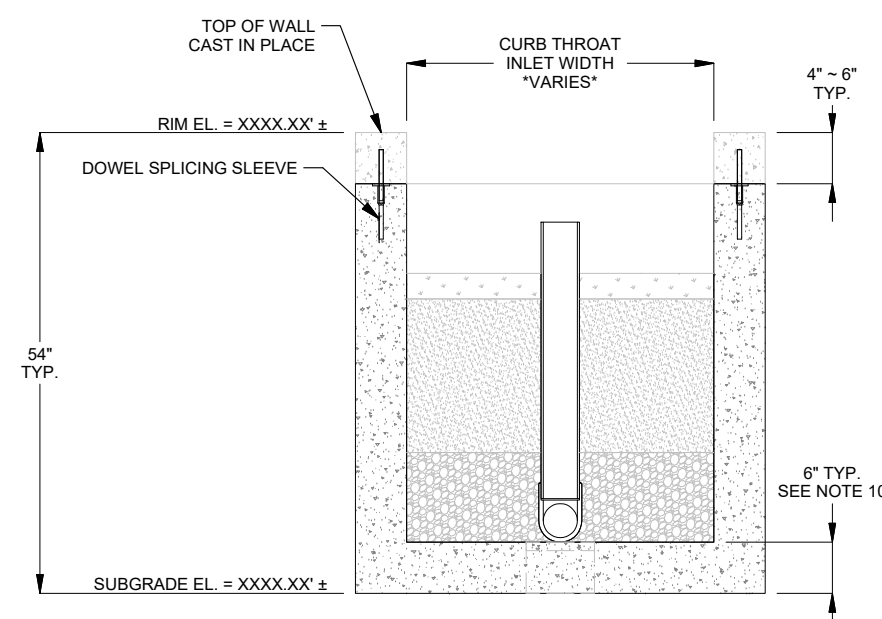
SECTION B-B
