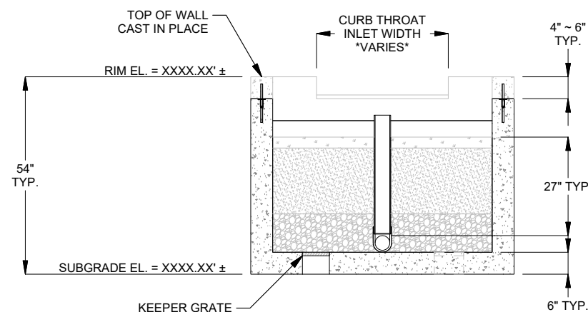
SECTION B-B
