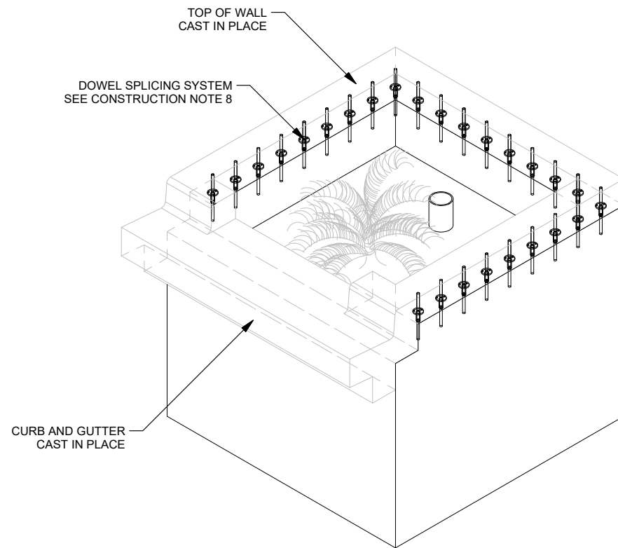
ISOMETRIC VIEW
