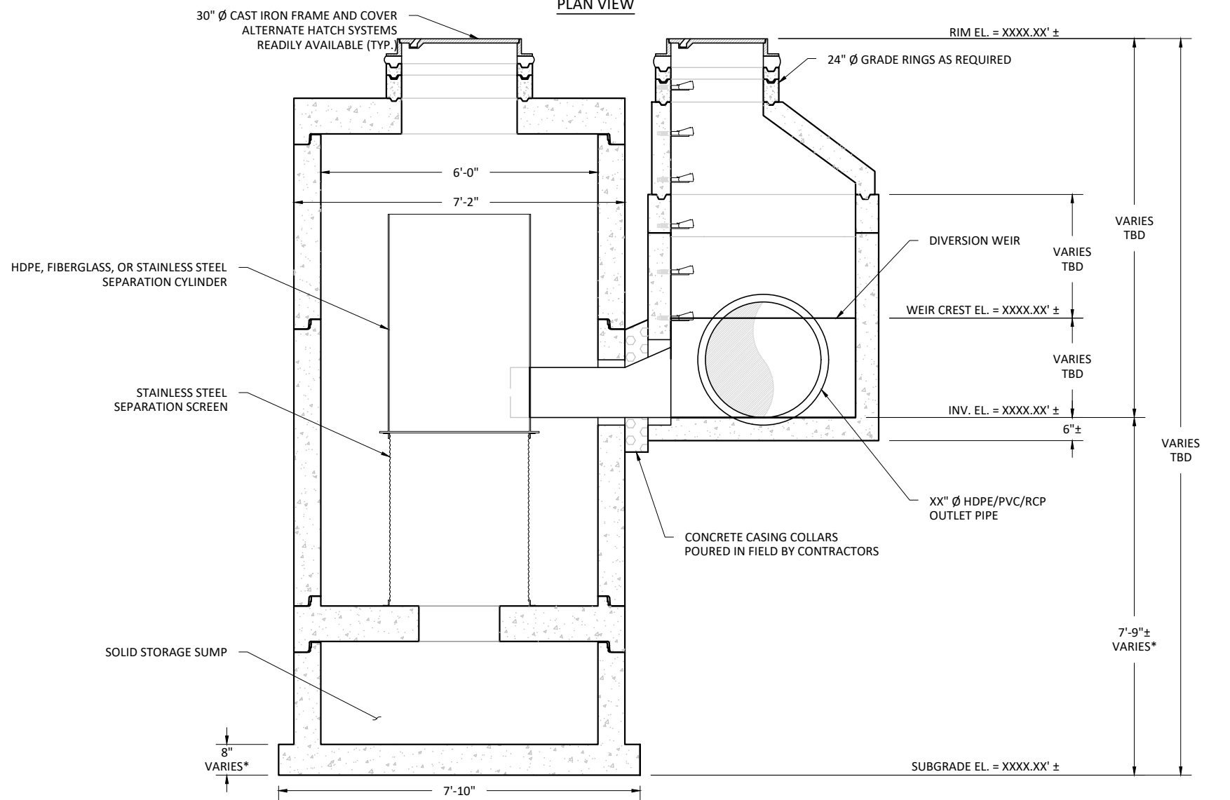
ELEVATION VIEW
