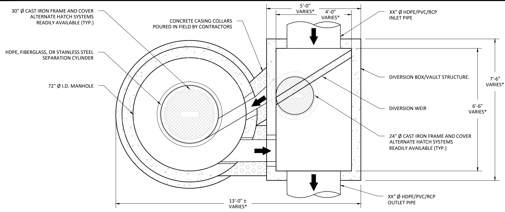
PLAN VIEW
