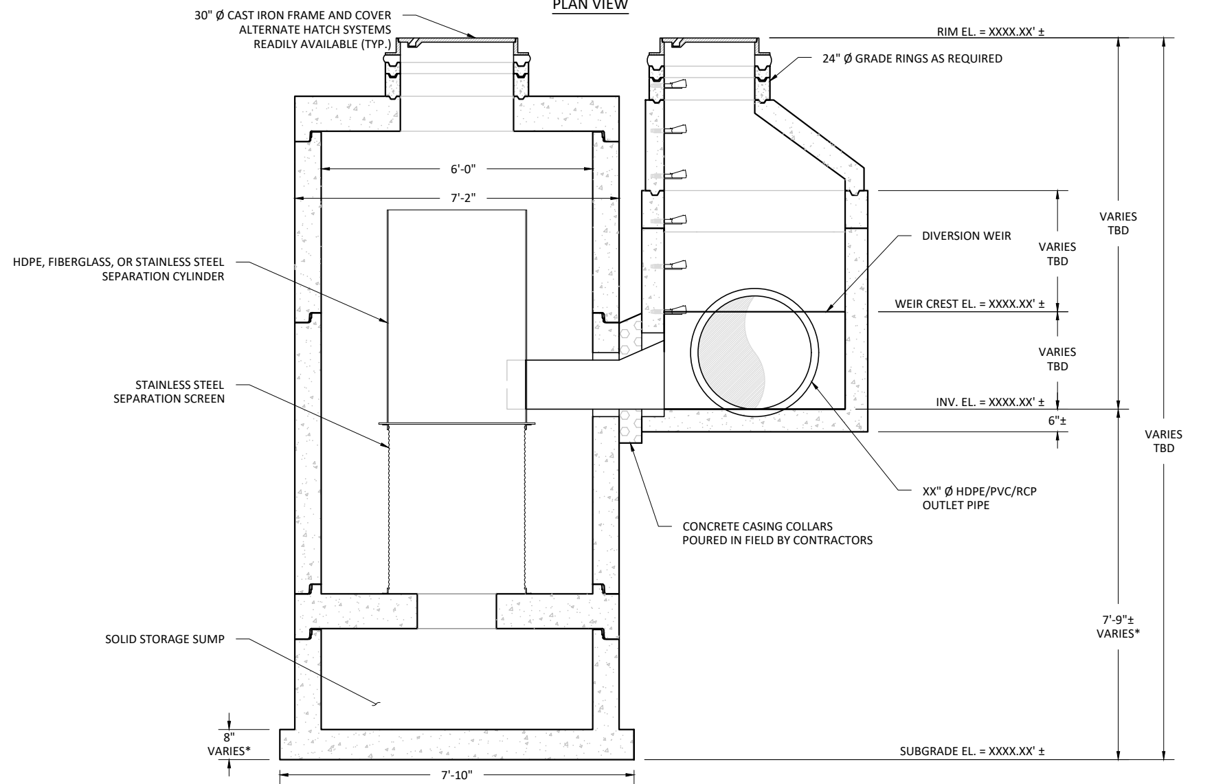
ELEVATION VIEW
