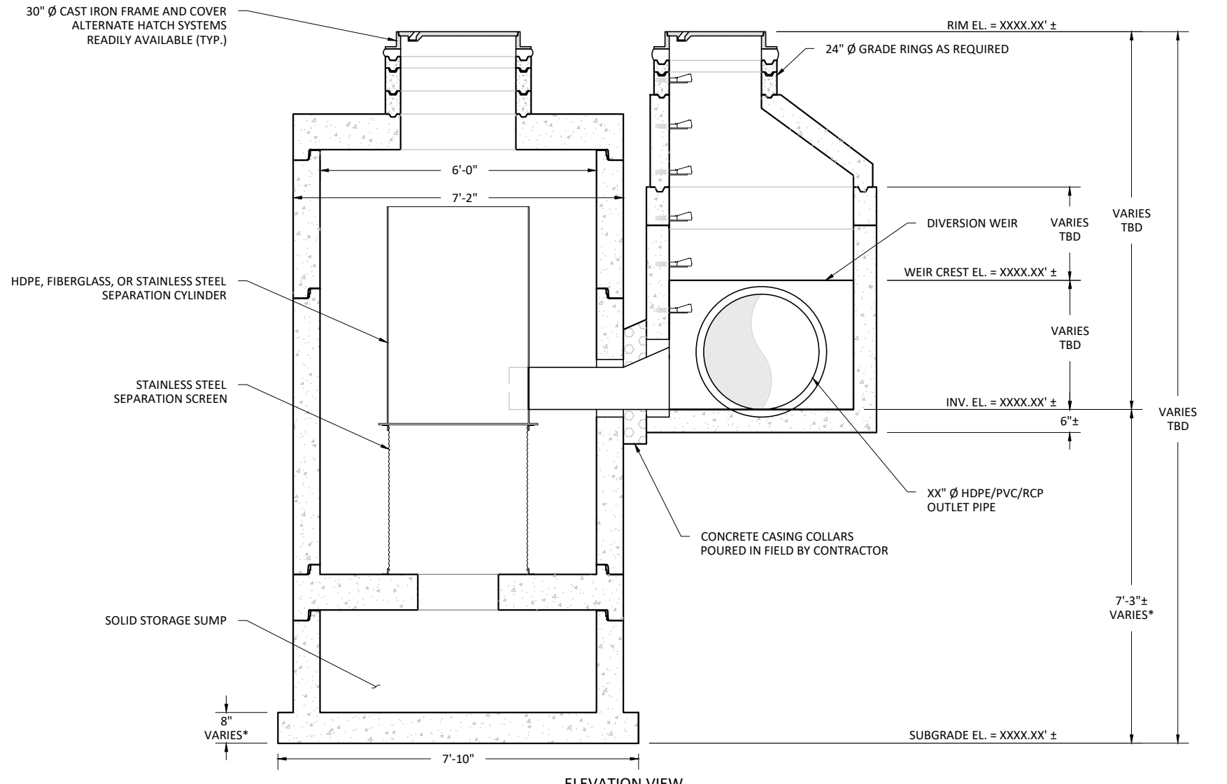
ELEVATION VIEW
