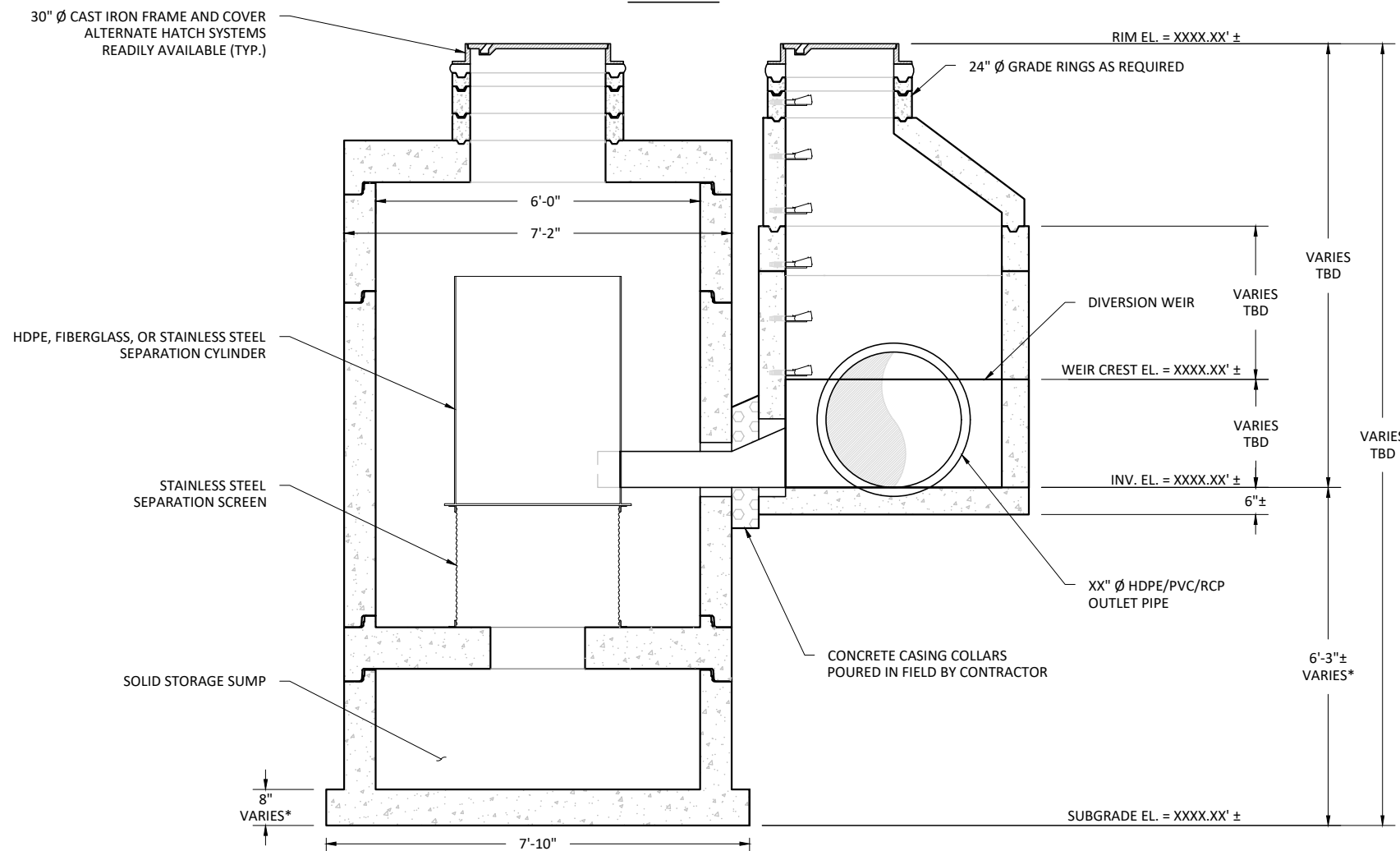
ELEVATION VIEW
