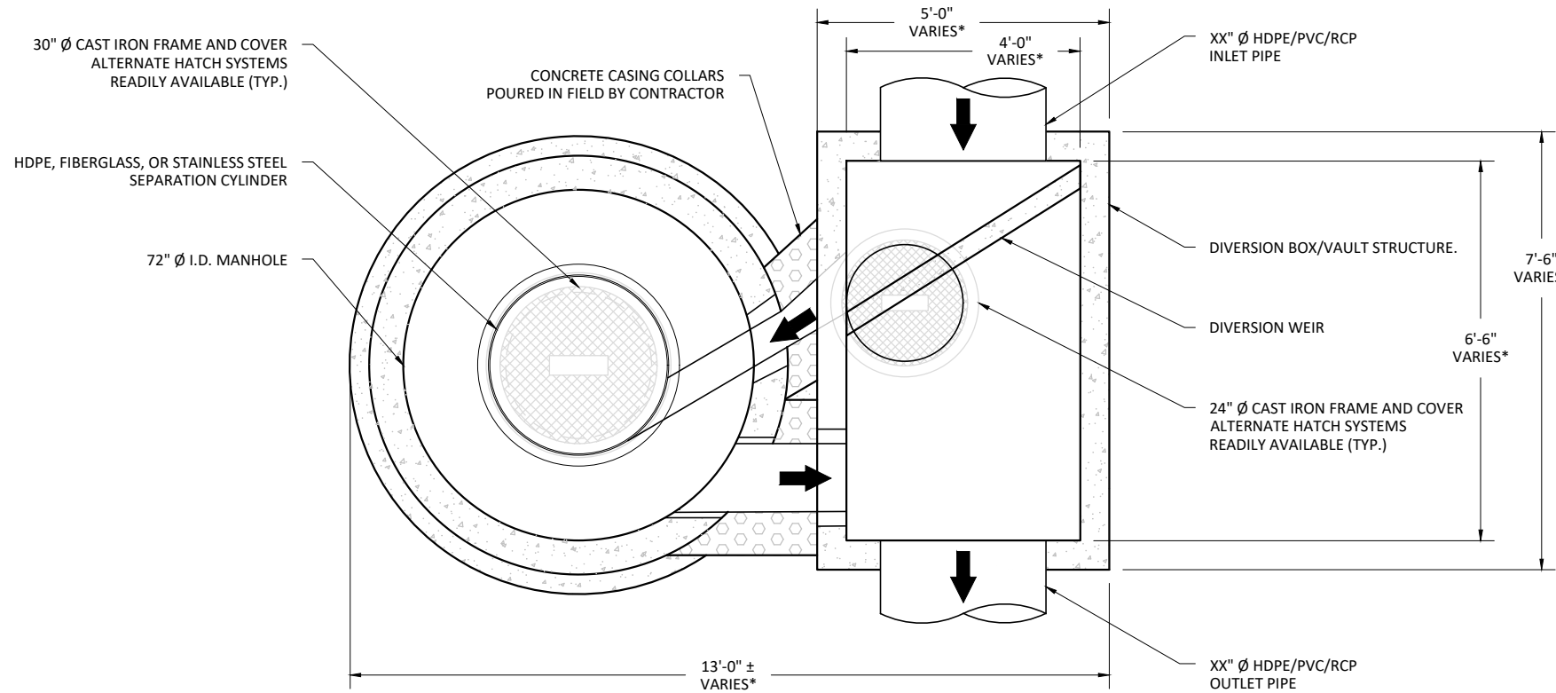
PLAN VIEW
