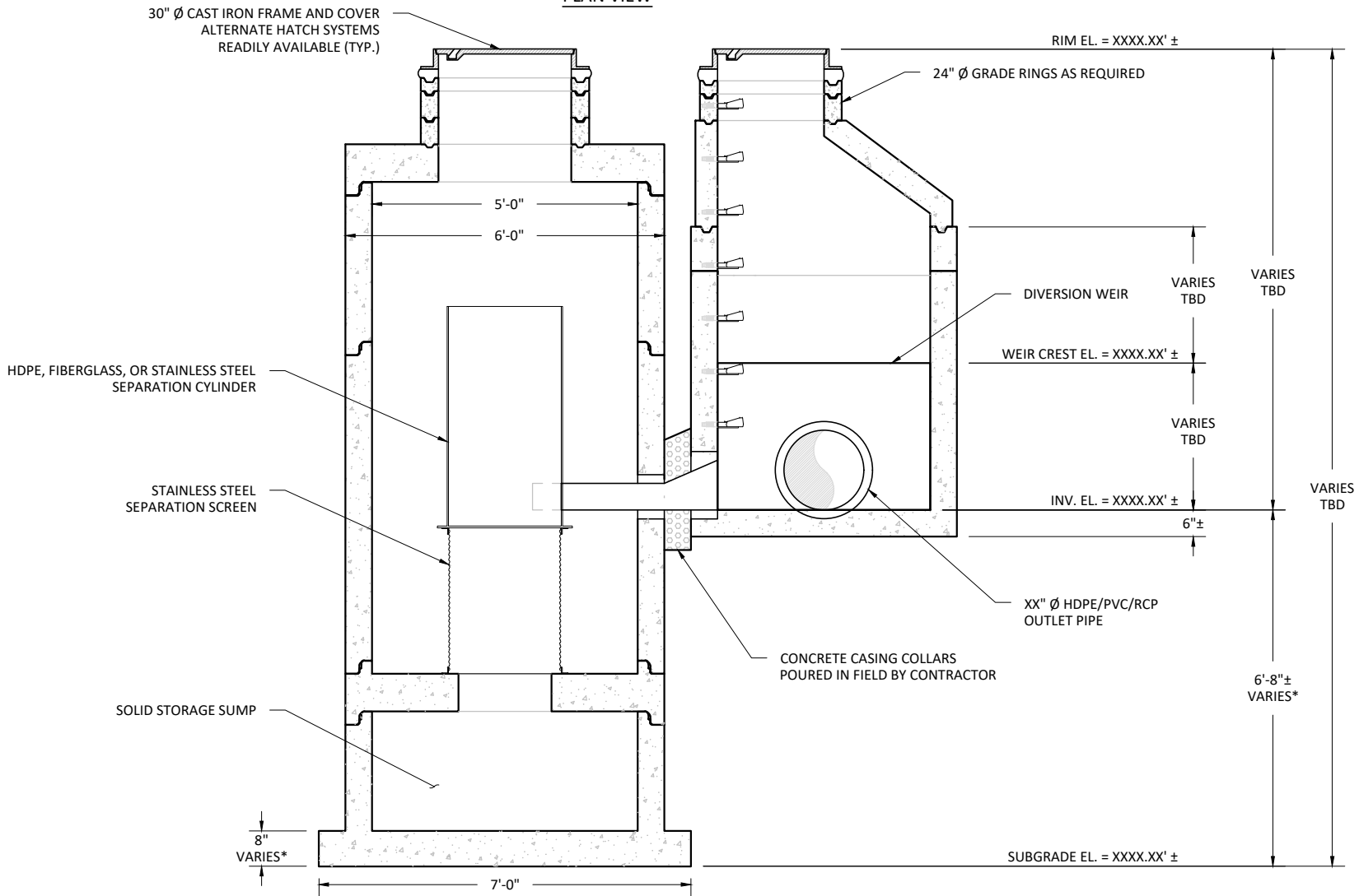
ELEVATION VIEW
