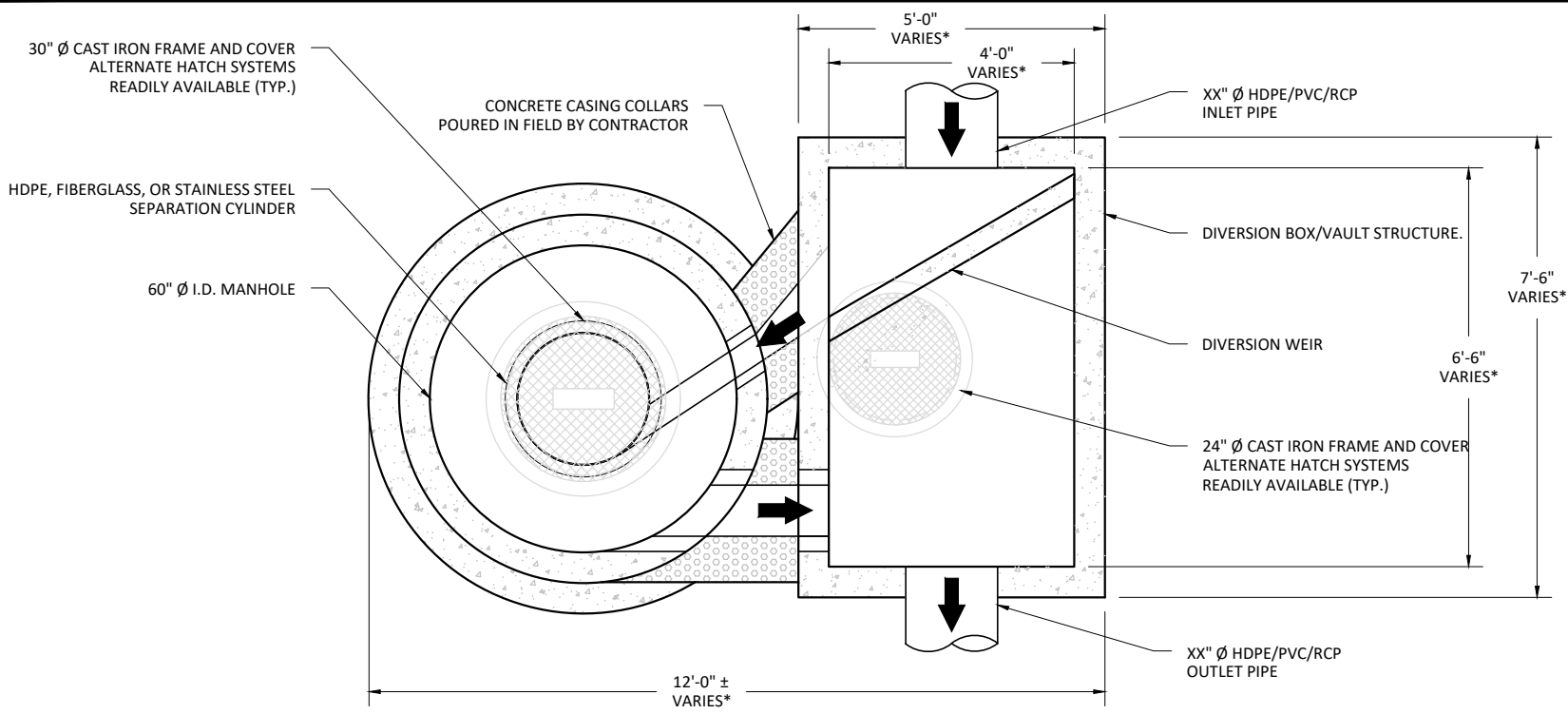
PLAN VIEW
