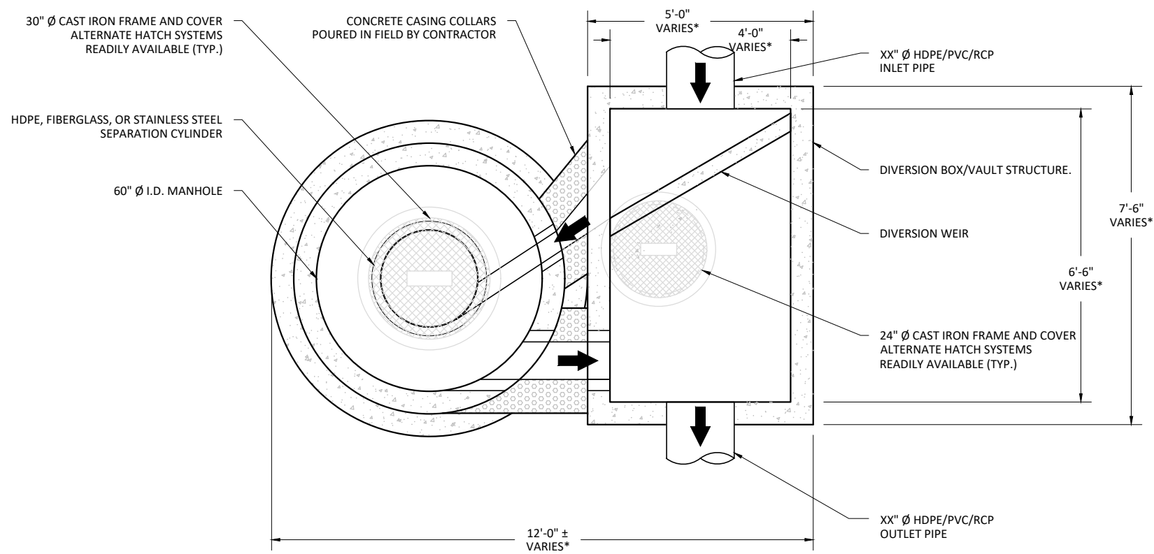
PLAN VIEW
