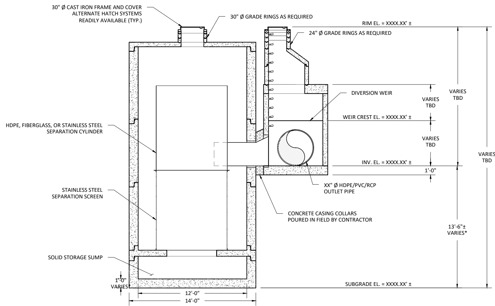
ELEVATION VIEW
