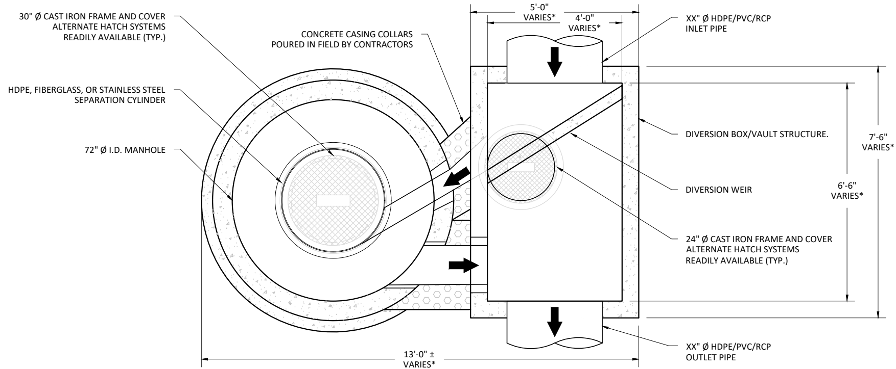
PLAN VIEW
