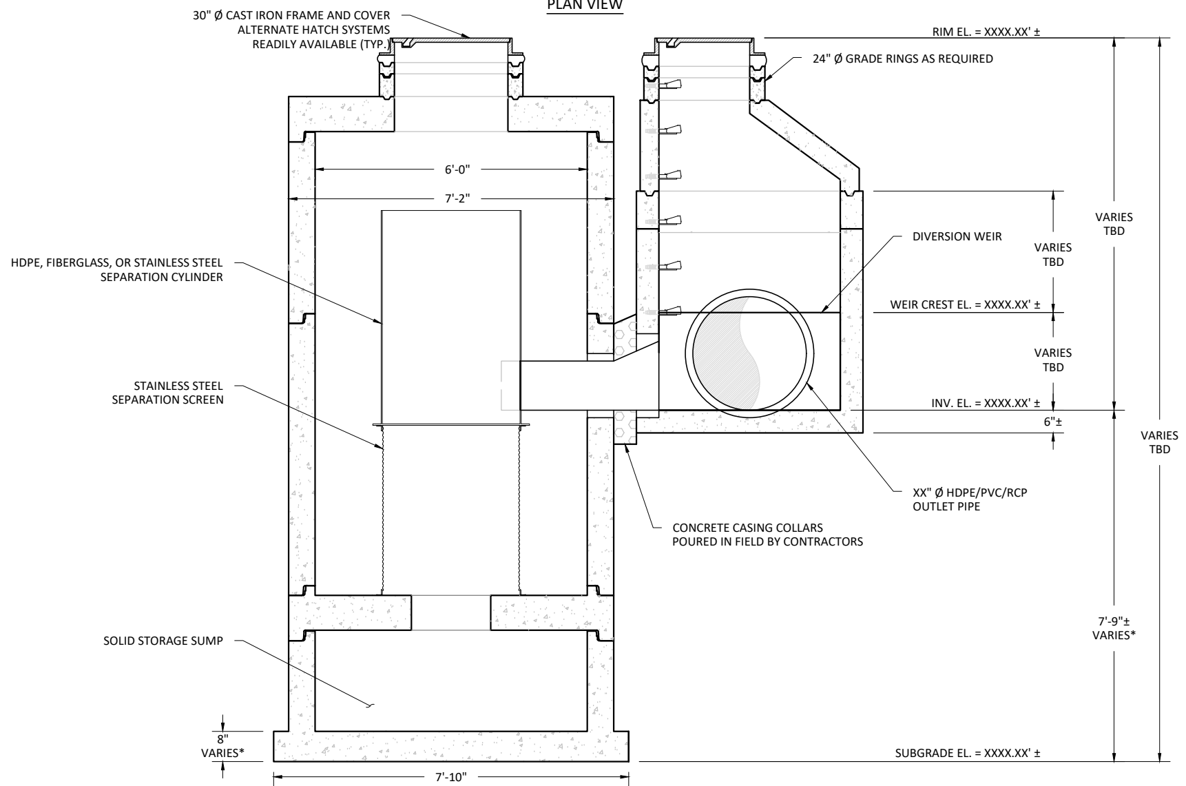
ELEVATION VIEW
