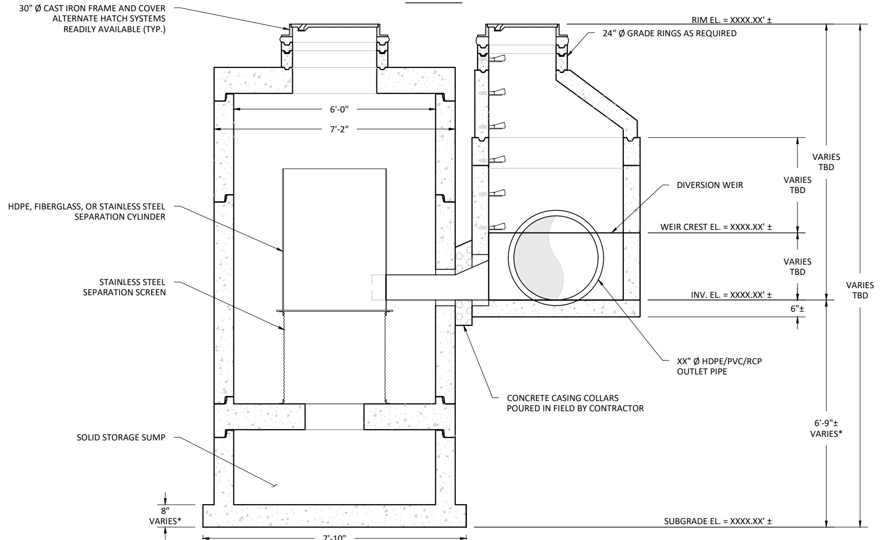
ELEVATION VIEW
