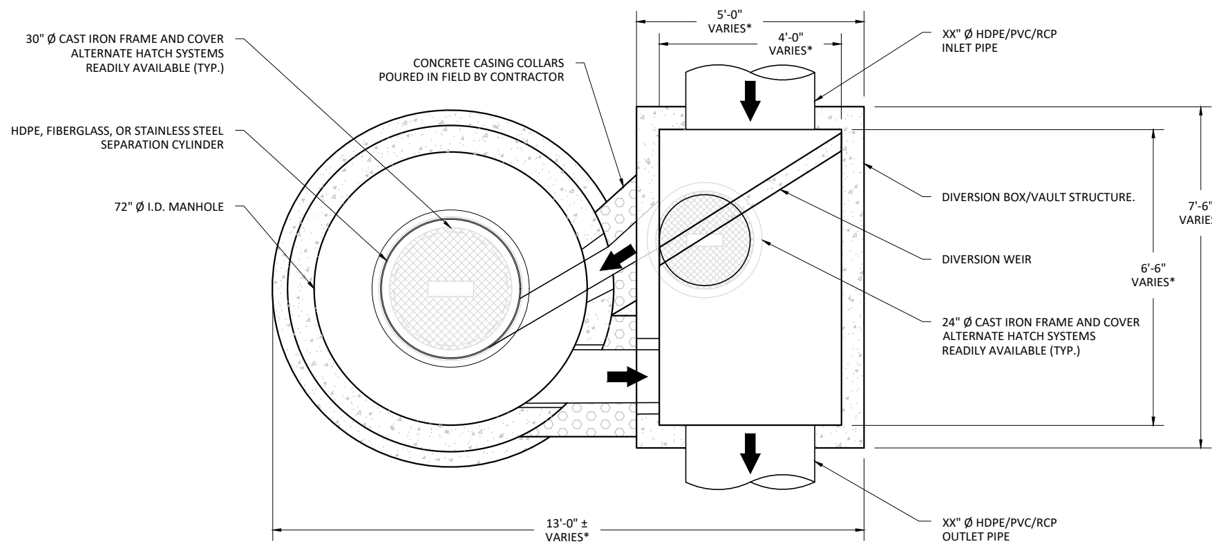
PLAN VIEW
