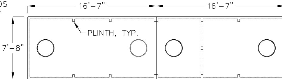
TOP VIEW JZ-8000
