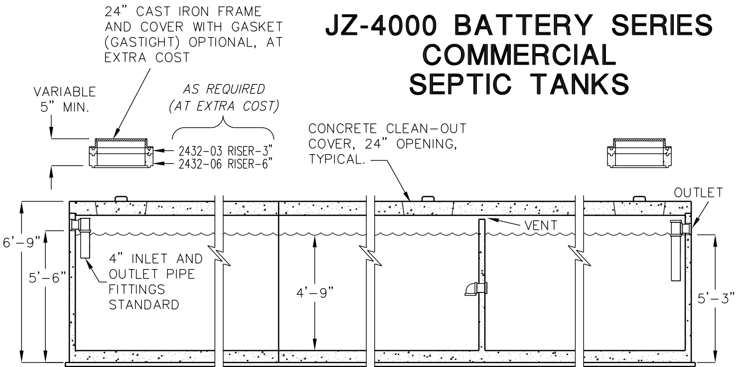
SIDE VIEW (CUT AWAY)
