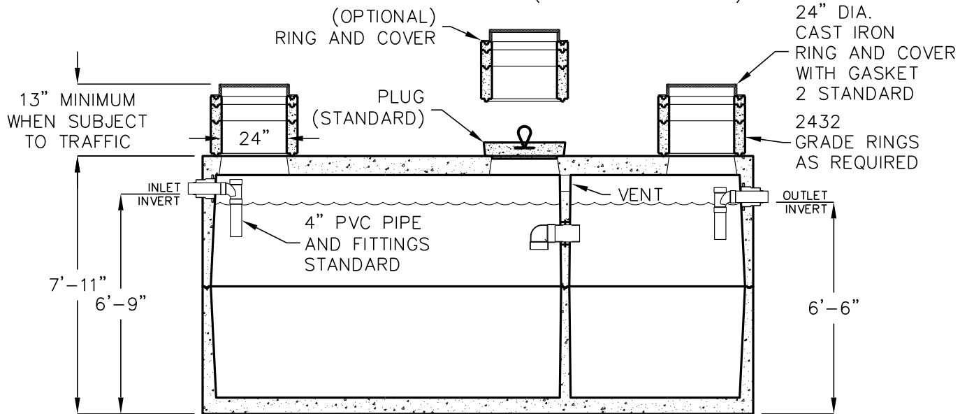
ELEVATION SECTION
