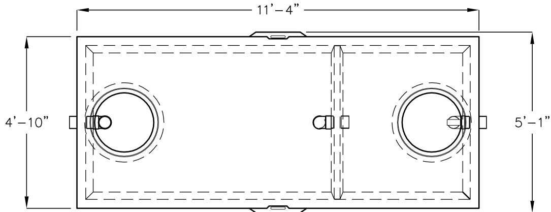
PLAN VIEW (COVERS NOT SHOWN)
