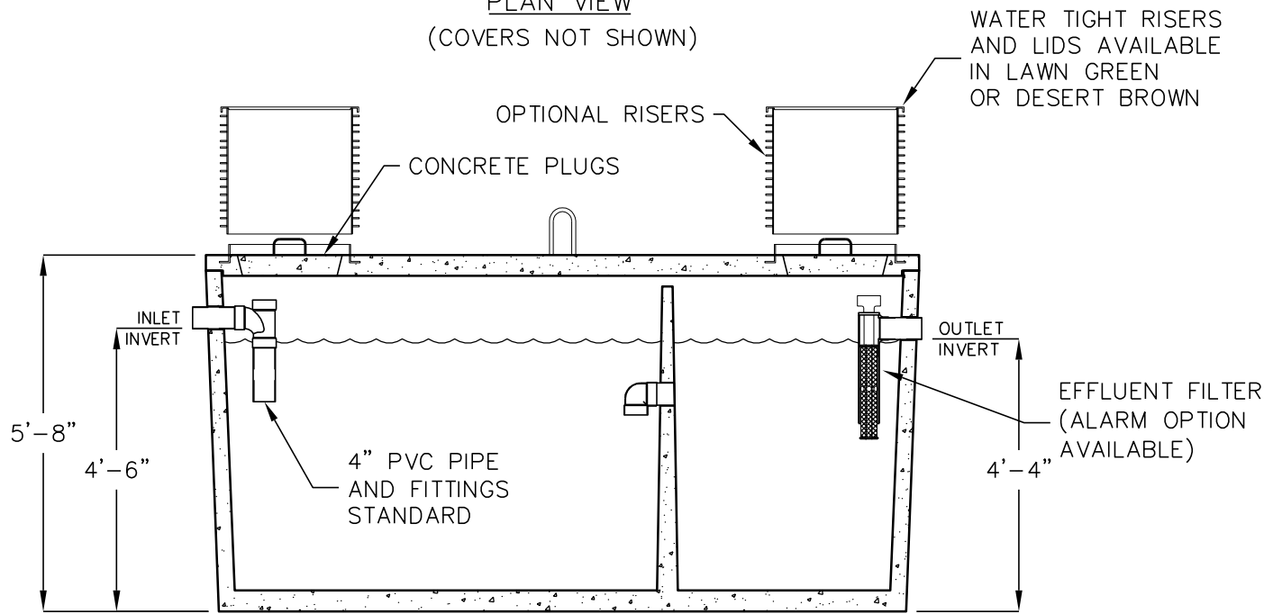
ELEVATION SECTION
