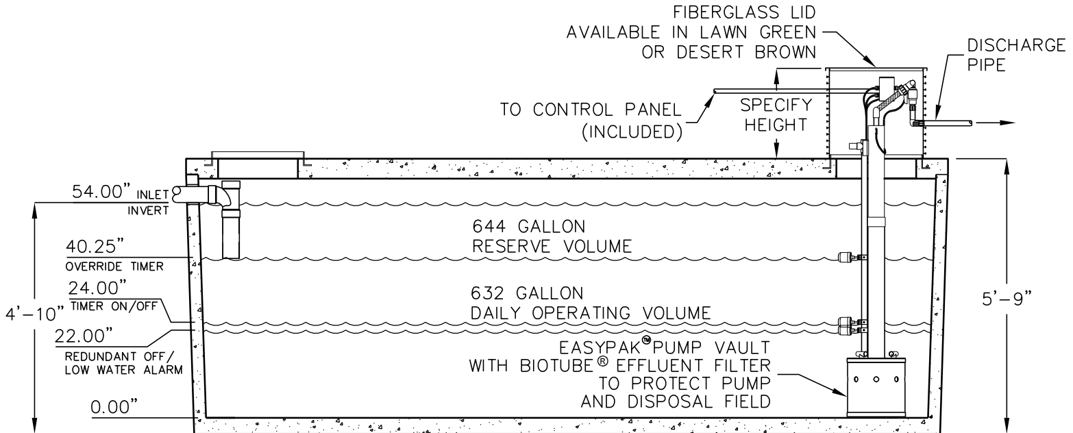
ELEVATION SECTION
