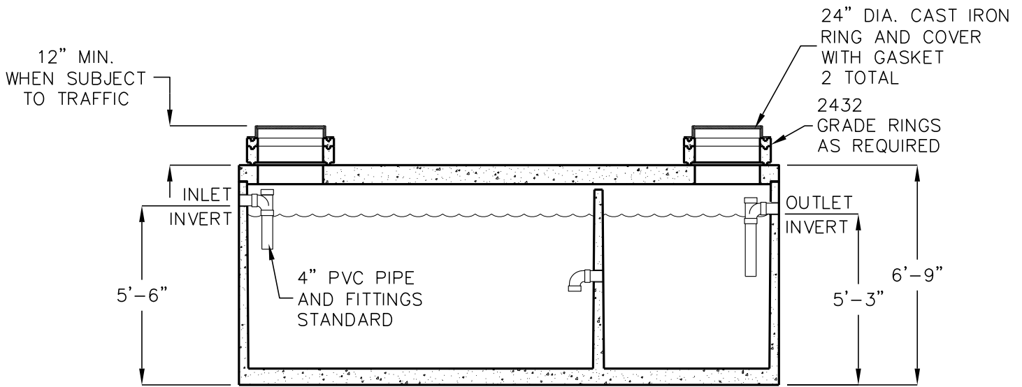
ELEVATION SECTION
