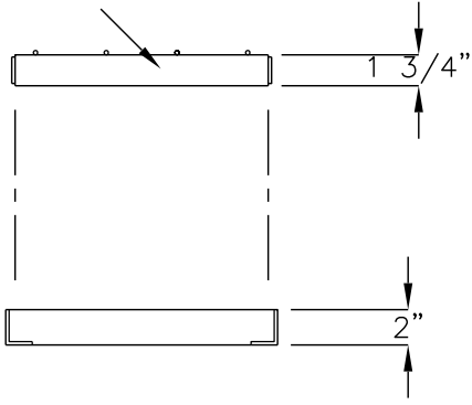
1212H GALVANIZED FRAME AND GRATE
