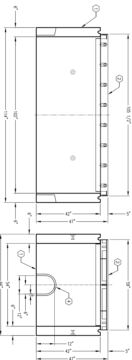
SECTION C-C
