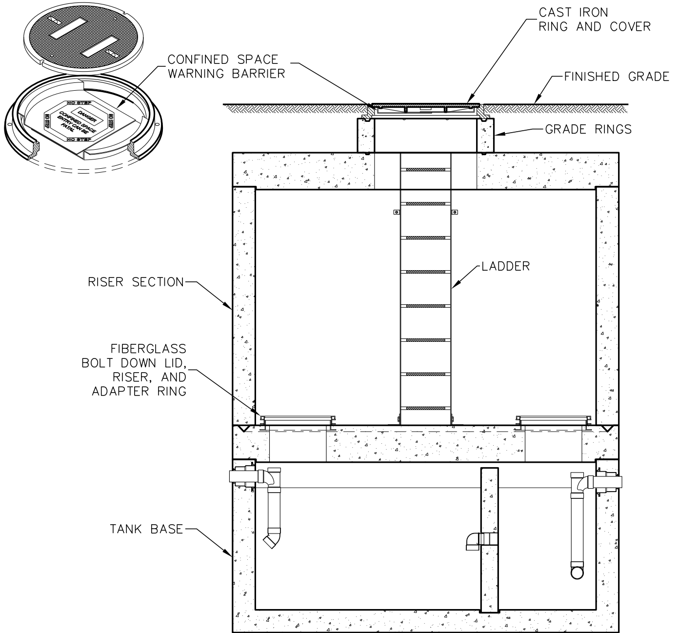
ELEVATION SECTION
