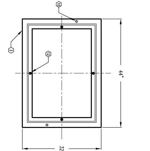
PLAN VIEW TOP SECTION
