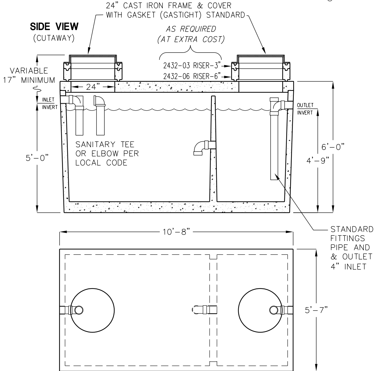
TOP VIEW (COVERS & RISERS REMOVED)
