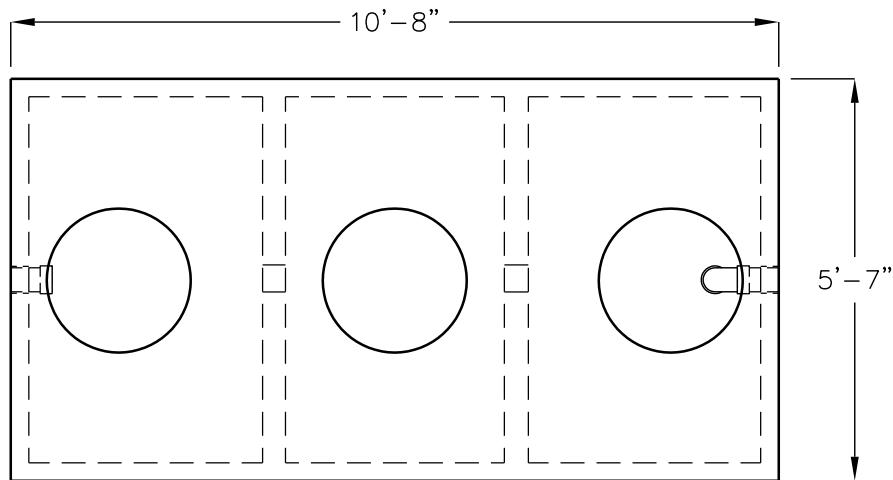
TOP VIEW (COVERS & RISERS REMOVED)
