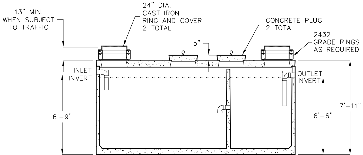
ELEVATION SECTION
