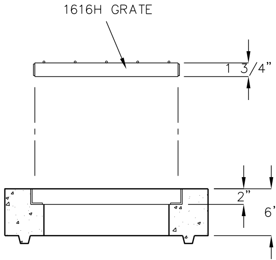
EXTENSION WITH CAST-IN FRAME SHOWN
