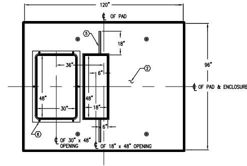
PLAN VIEW OF TRANSFORMER PAD
