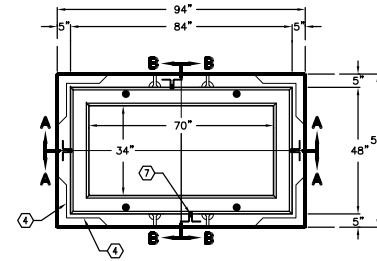
PLAN VIEW W/O TRANSFORMER PAD
