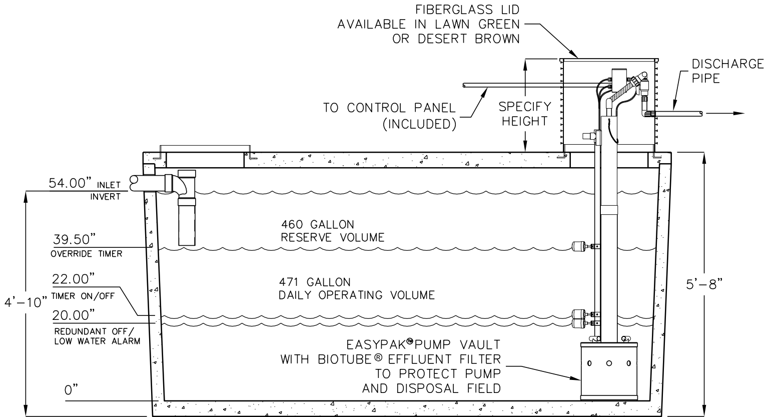
ELEVATION SECTION
