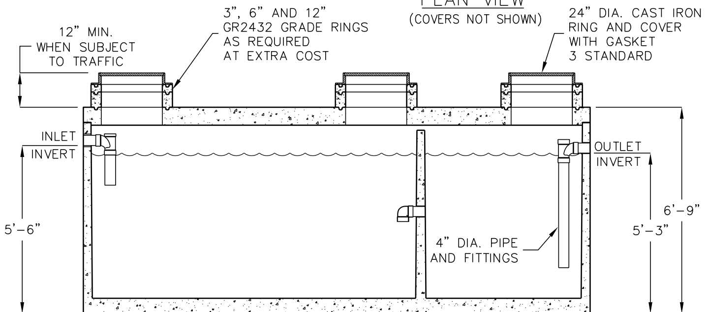
ELEVATION SECTION
