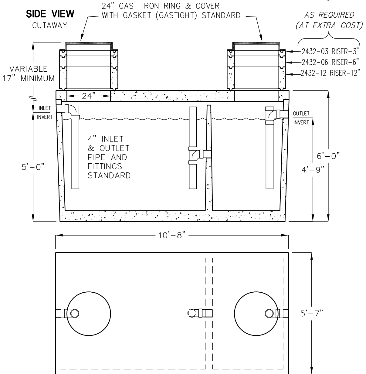
TOP VIEW (COVERS & RISERS REMOVED)
