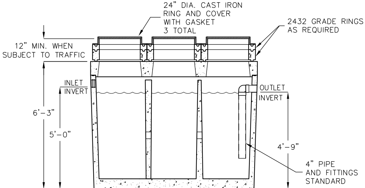
ELEVATION SECTION
