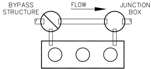
STORMWATER INTERCEPTOR TYPICAL SYSTEM CONFIGURATION (SEE NOTE 1)
