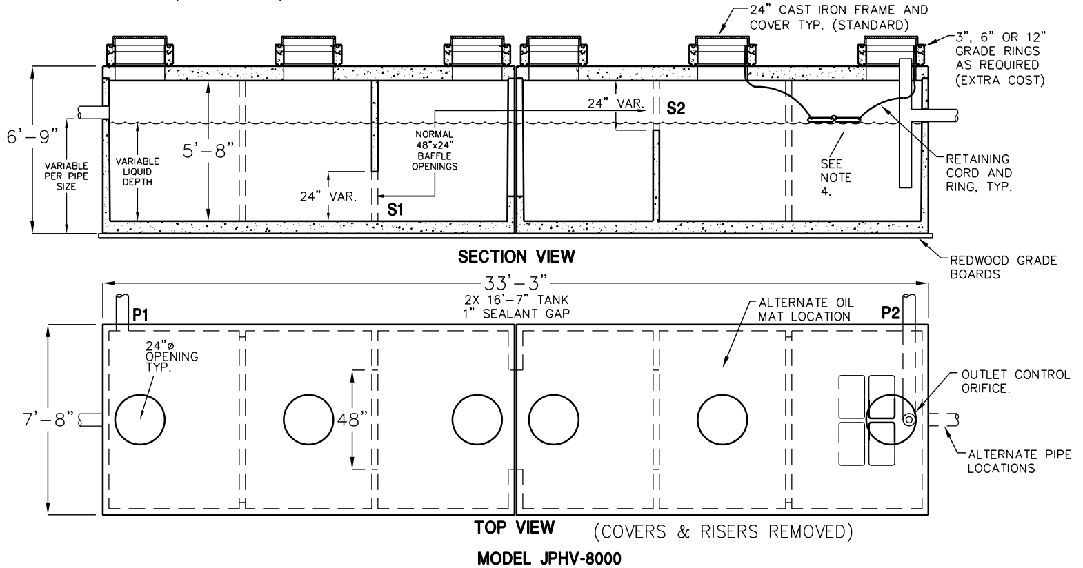
STORMWATER INTERCEPTOR TYPICAL SYSTEM CONFIGURATION (SEE NOTE 1)
