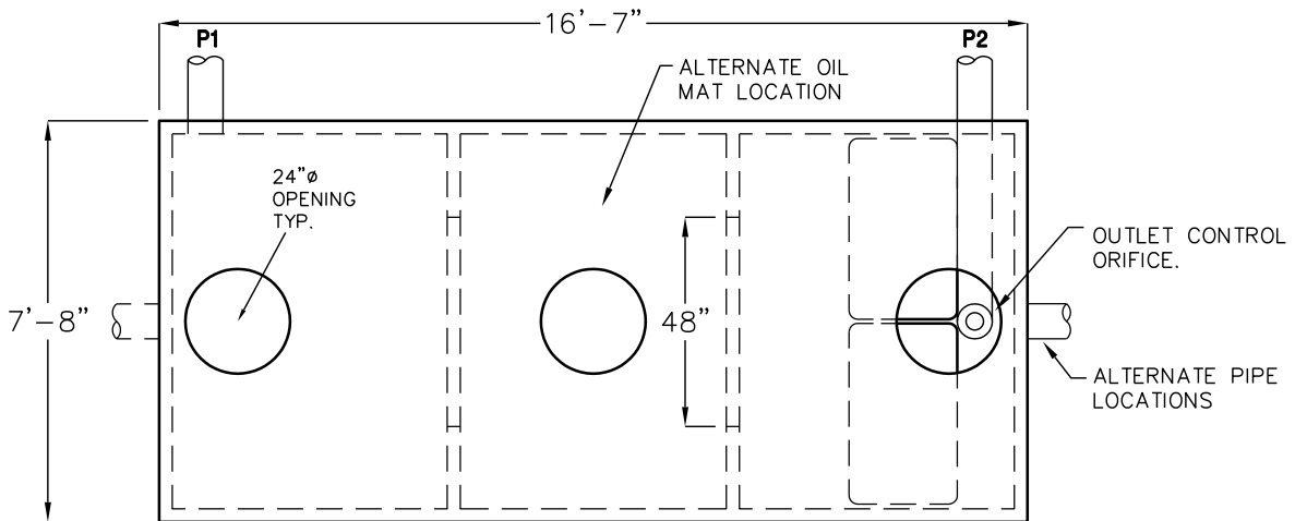
TOP VIEW (COVERS & RISERS REMOVED)
