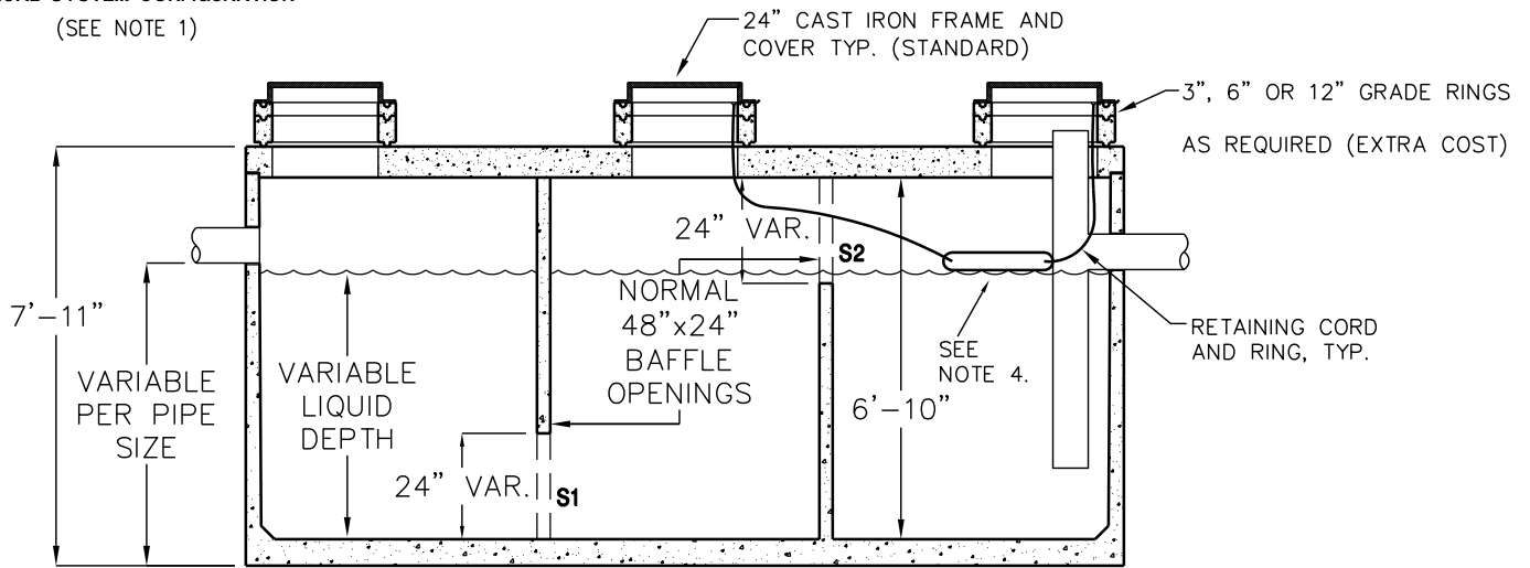
SECTION VIEW
