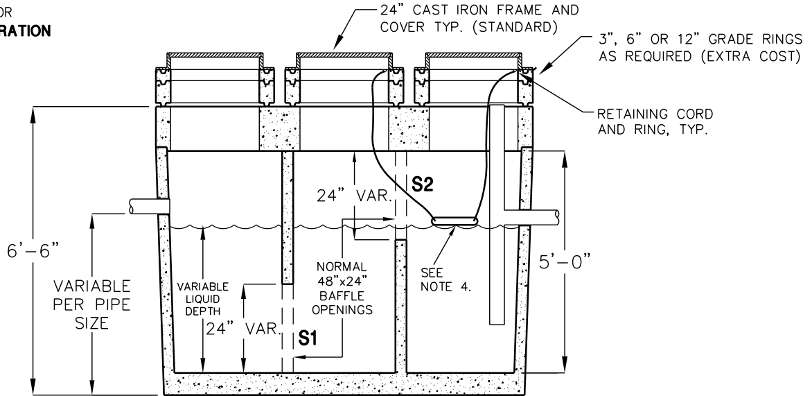
SECTION VIEW
