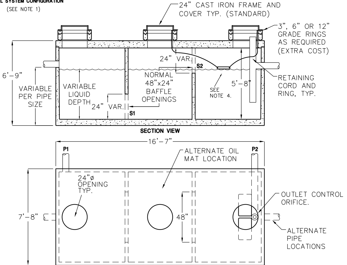
STORMWATER INTERCEPTOR TYPICAL SYSTEM CONFIGURATION (SEE NOTE 1)
