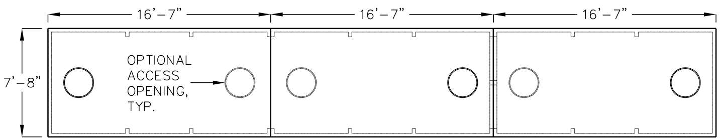
TOP VIEW JZ-15000
