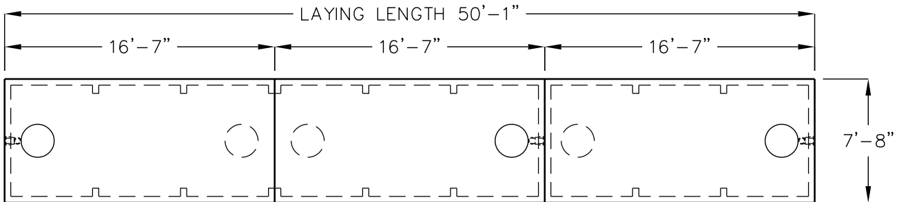
TOP VIEW (COVERS REMOVED)
