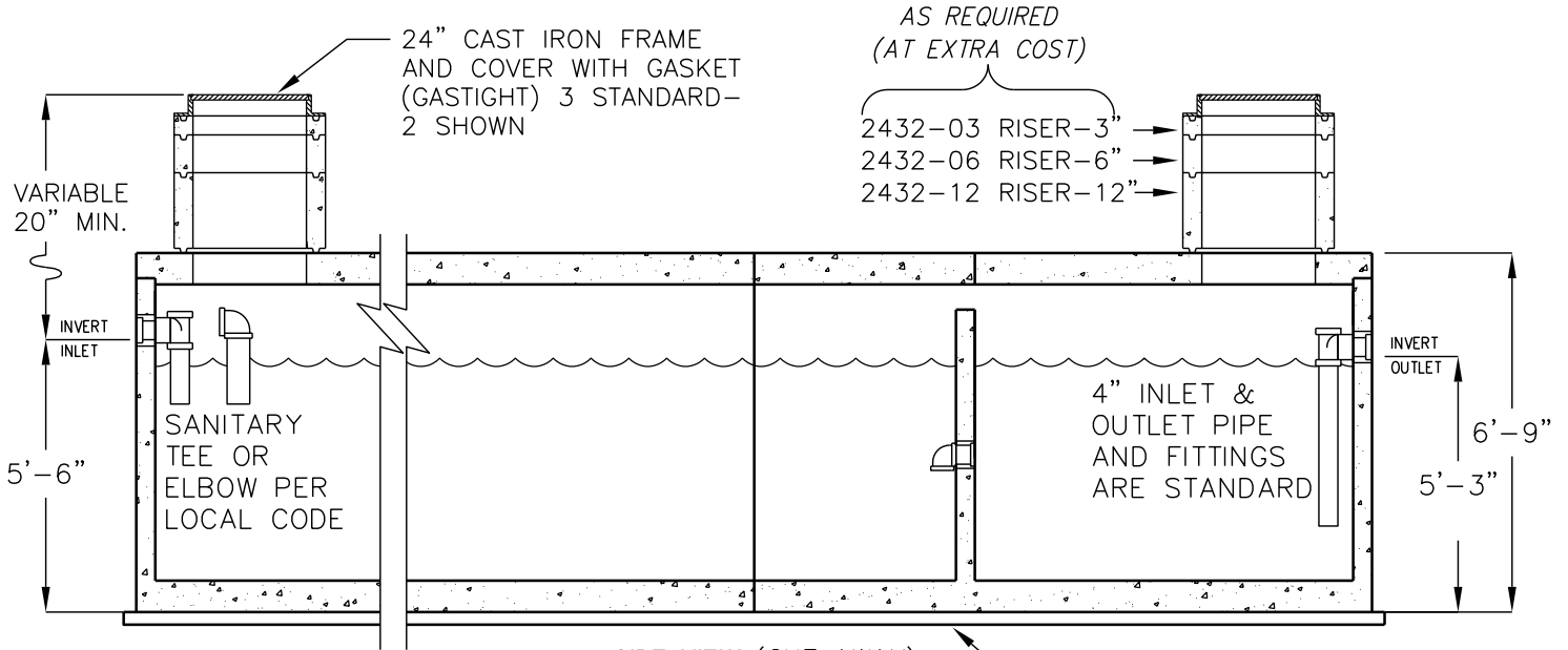
SIDE VIEW (CUT AWAY)
