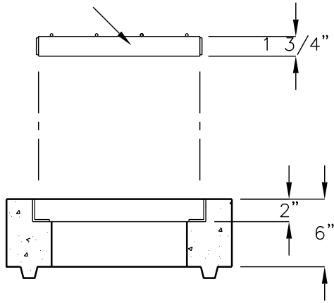
EXTENSION WITH CAST-IN FRAME SHOWN
