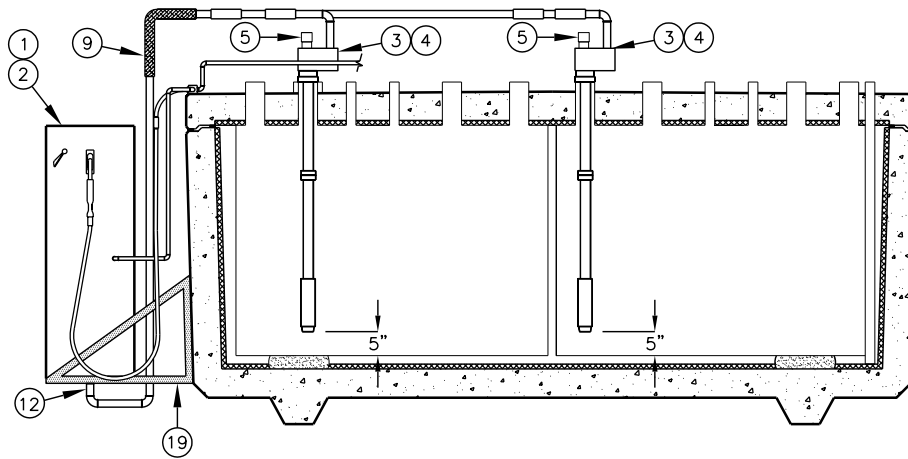
ELEVATION (CUTAWAY)
