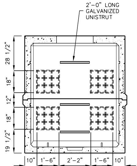
TYPICAL END VIEW
