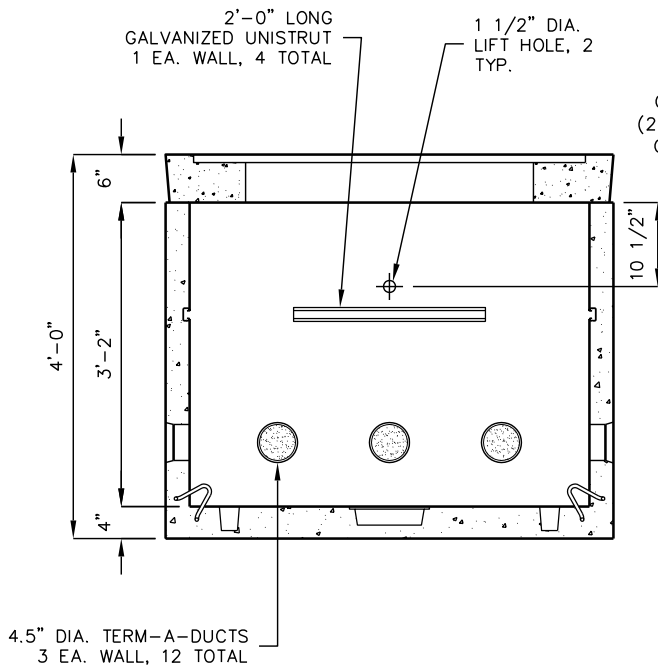
TYPICAL SIDE VIEW
