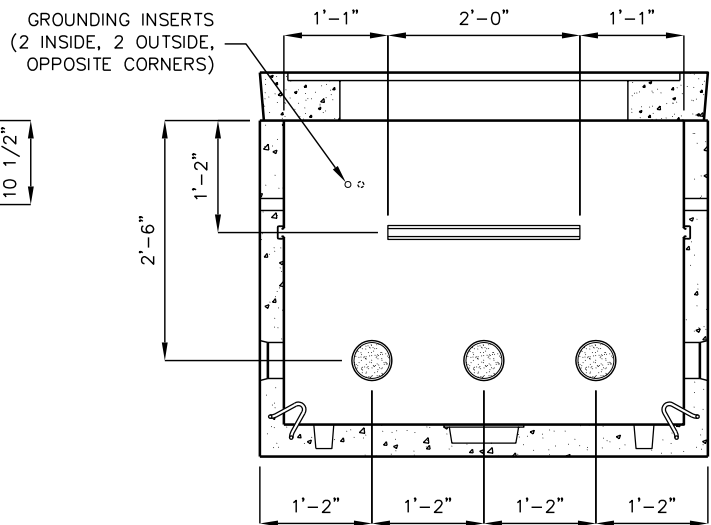
TYPICAL END VIEW
