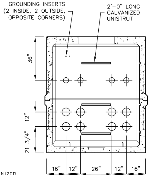
TYPICAL END VIEW
