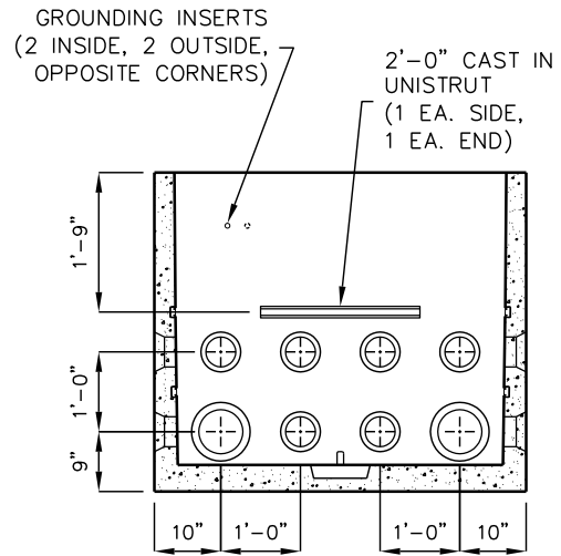
END VIEW (TYP.)
