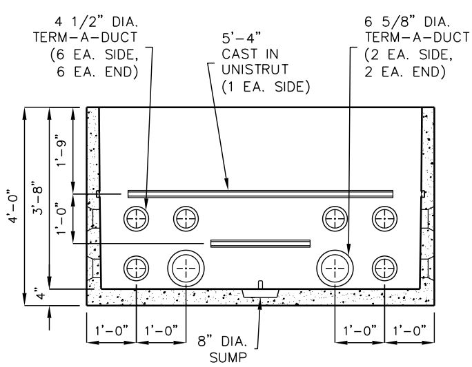
SIDE VIEW (TYP.)
