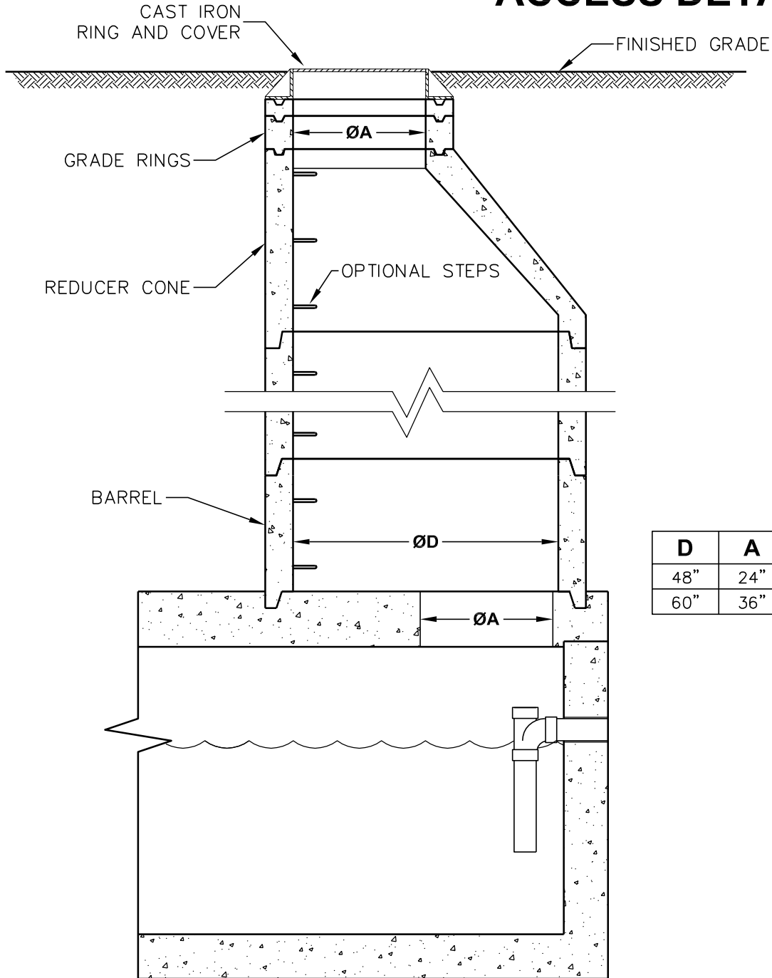
ELEVATION SECTION VIEW
